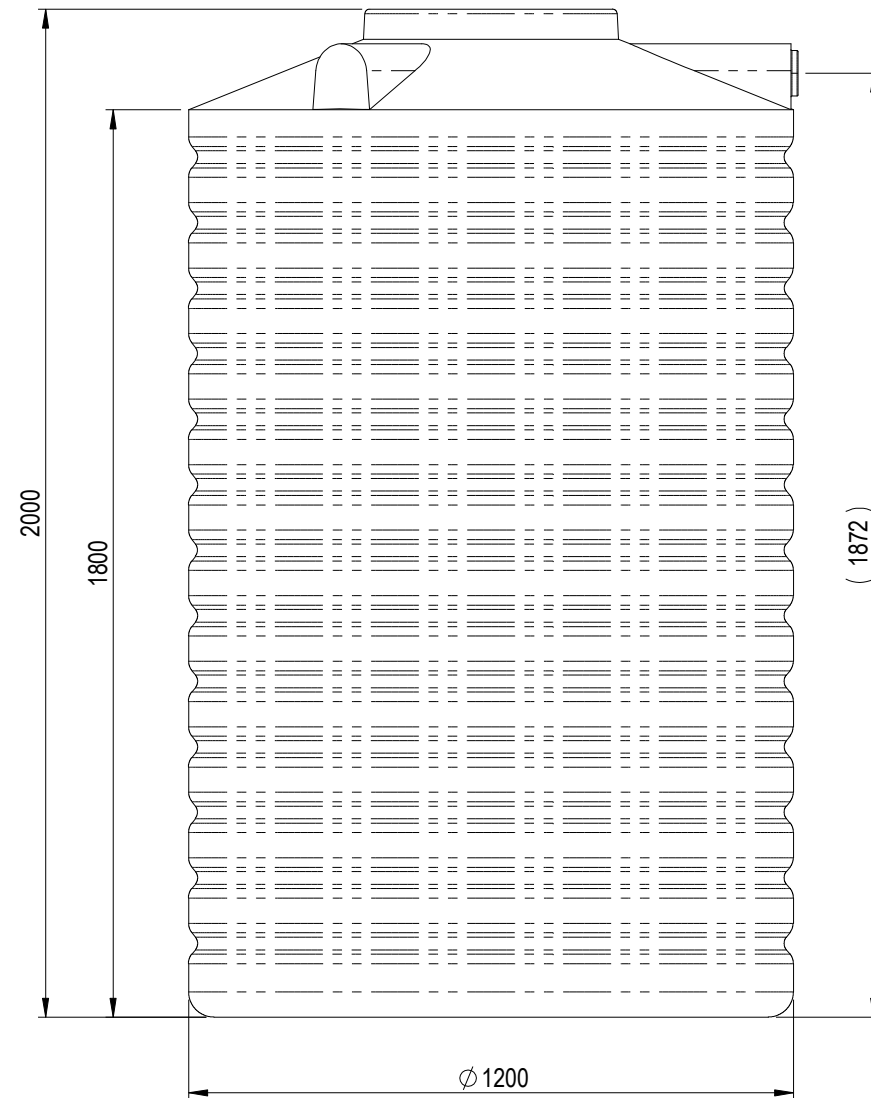
FRONT VIEW
